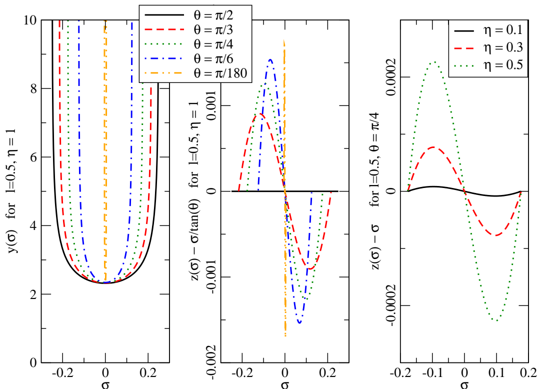
Figure 4: Solutions y(\sigma) , z(\sigma) of the differential equations (5.7) and (5.8) with boundary conditions (5.3) for different orientation angles \theta and rapidity \eta . These solutions characterize the two-dimensional world sheet bounded by the Wilson loop. For definitions, see figure 3 and text. Left panel: y(\sigma) for \eta = 1 for varying \theta . Middle panel: z(\sigma) - \sigma/\tan\theta for \eta = 1 for varying \theta . As figure 3 illustrates, z(\sigma) - \sigma/\tan\theta would be zero if the projection of the string onto the D3-brane at y = \Lambda were a straight line. Third panel: z(\sigma) - \sigma/\tan\theta for \theta = \pi/4 for varying \eta .
